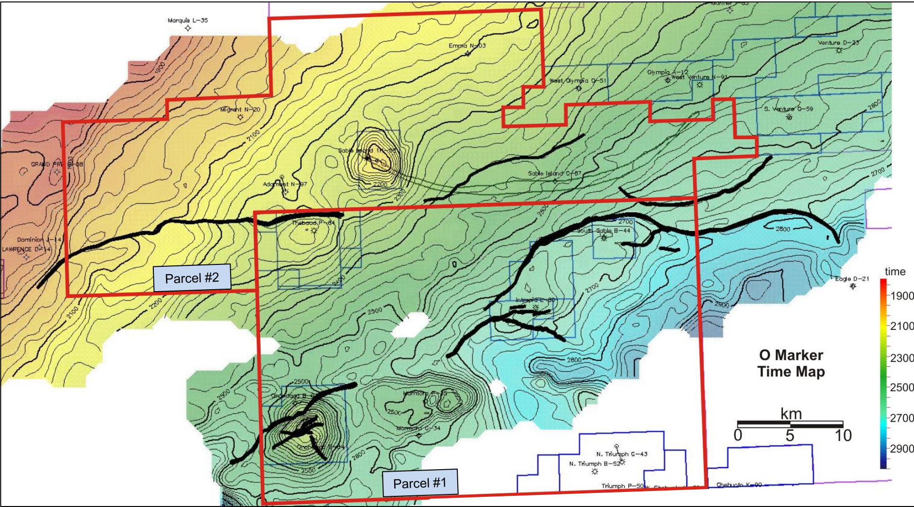
Time Structure Map of Early Cretaceous (Barremian to Hauterivian) 'O' Seismic Marker. The existing Significant and Commercial Discovery Areas are outlined in blue. Note the areas covered by the existing discoveries are not part of the land description for the Parcels.
